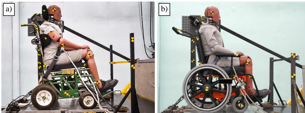
Figure 4. a) Tiedown/securement system testing using surrogate wheelchair [19], b) Example of wheelchair frontal-impact testing [20].
