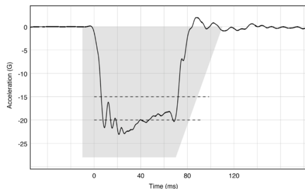
Figure 6. Typical 30-mph sled deceleration pulse [21]
