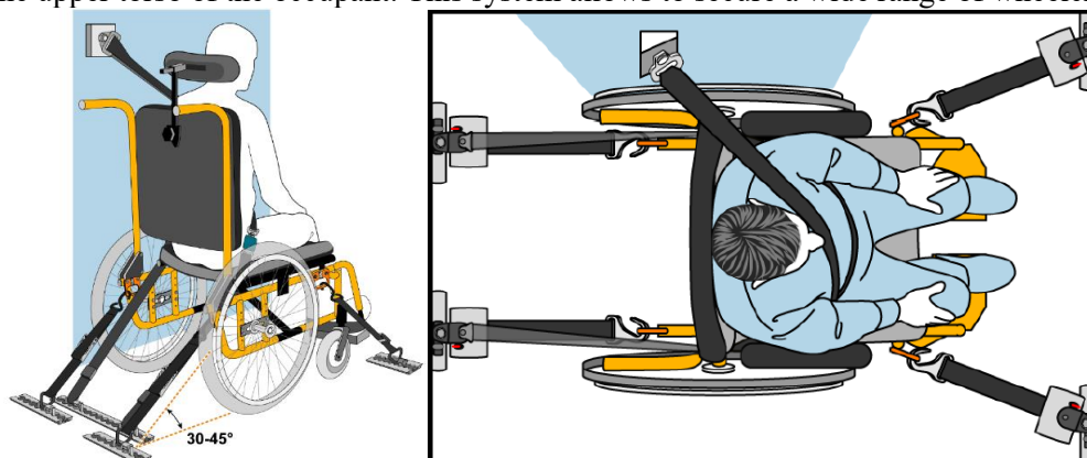
Figure 1. Wheelchair Tie-down and Occupant Restraint System [11].
